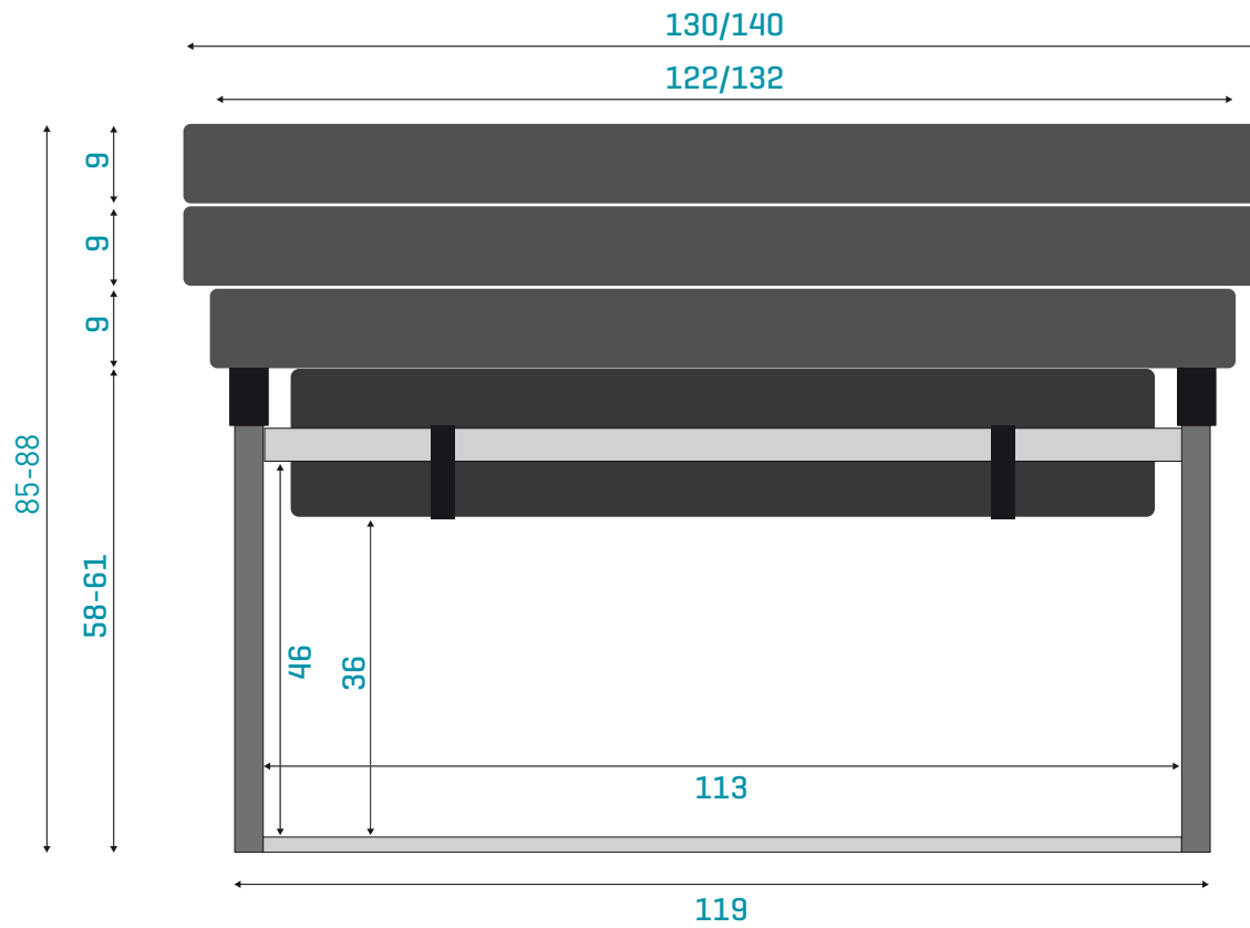
FRONT VIEW
