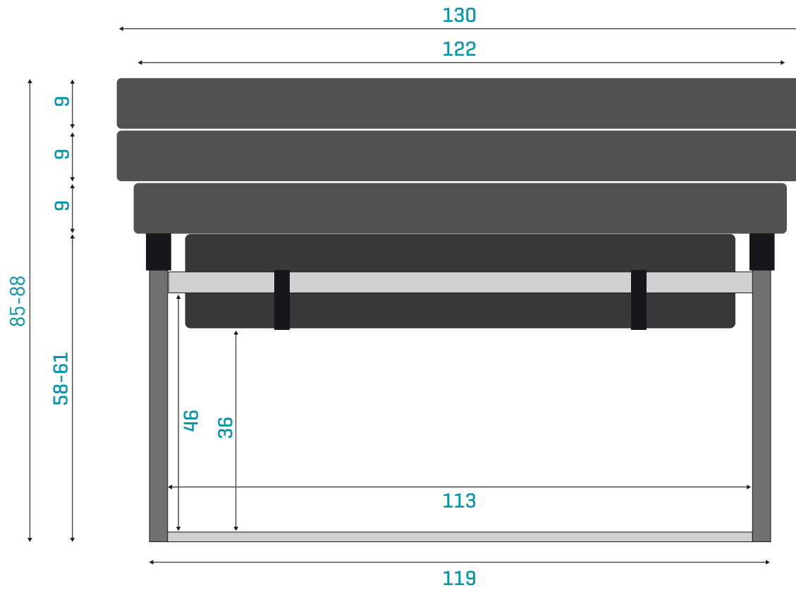
FRONT VIEW
